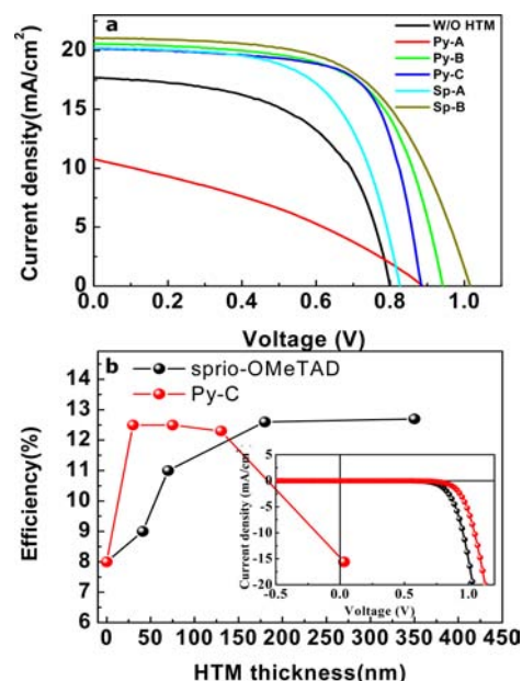
Figure 4. (a) Current density–voltage ( J – V ) curves for TiO 2 /MAPbI 3 /HTMs/Au fabricated with Py-A, Py-B, Py-C, Sp-A, and Sp-B as HTMs, and without HTM. (b) The efficiency dependence on the overlayer thickness with Py-C and spiro-OMeTAD; inset is dark J – V curves for Py-C and Sp-B devices.
